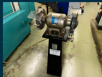
ALPINE Bench grinder on stand. 3000 rpm. 240 volts
